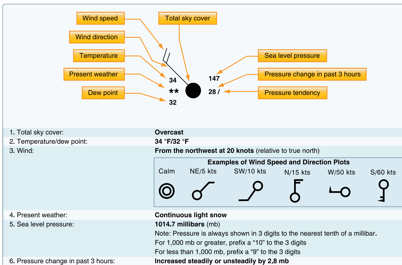
Figure 13-11. Sample station model and weather chart symbols.
